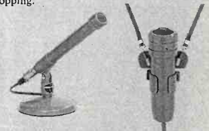
M-40 Studio Microphone, M-20 Lavalier Microphone — dynamic, omnidirectional microphones specifically designed for radio and television use. Smooth response over 60-18,000 cps frequency range.
